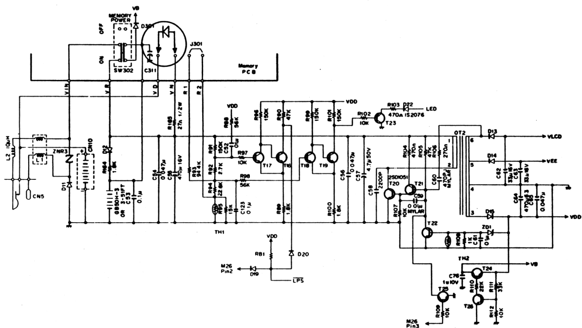
Figure 2. Power Supply Section of Main PCB.
