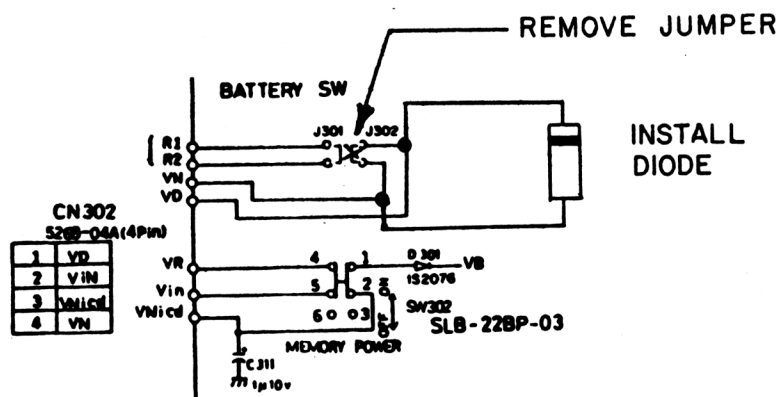
Figure 1. Memory PCB.
